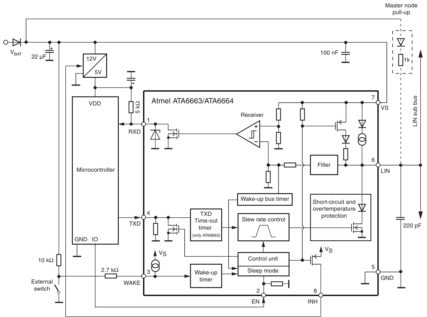
Figure 7-2. Application Circuit
